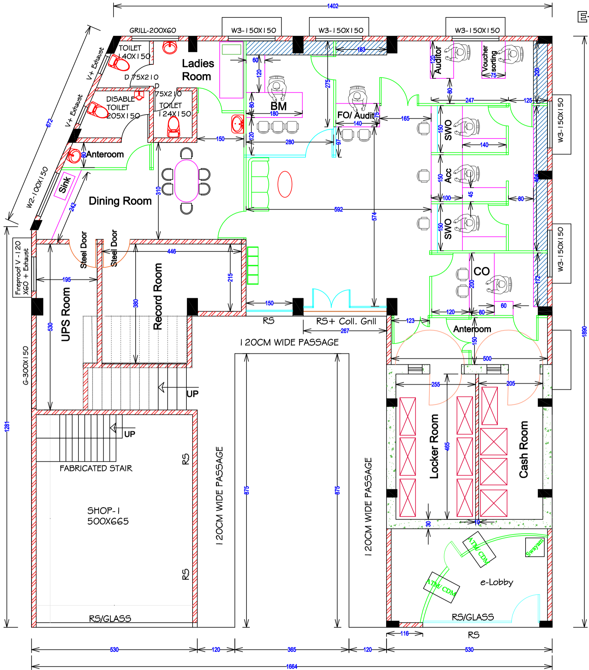
DESHAMANGALAM BRANCH - PROPOSED LAYOUT PLAN
